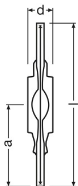
HQI-TS 70 W/WDL, HQI-TS 70 W/NDL, HQI-TS 70 W/D, HQI-TS 70 W/CD, HQI-TS 150 W/WDL, HQI-TS 150 W/NDL, HQI-TS 150 W/D, HQI-TS 150 W/CD
